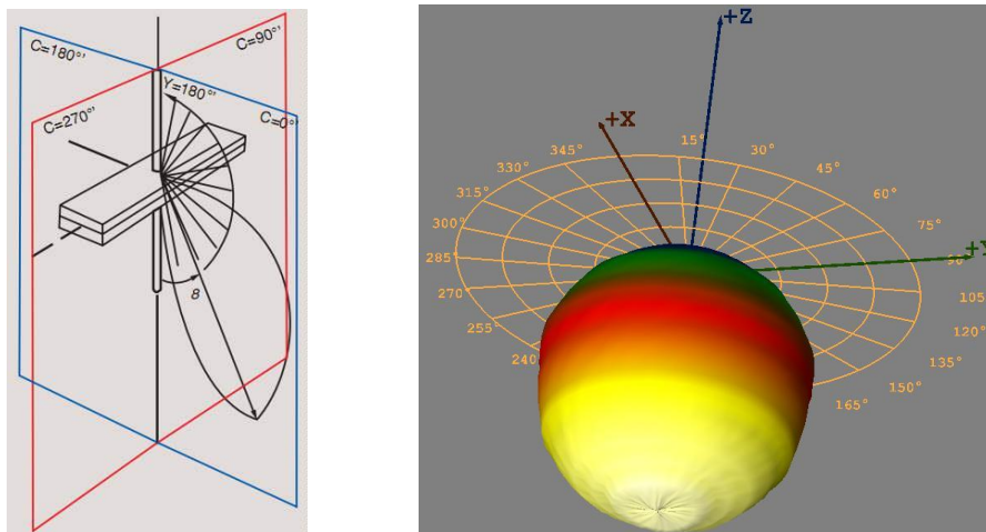
Luminaire light distribution of the 3D
